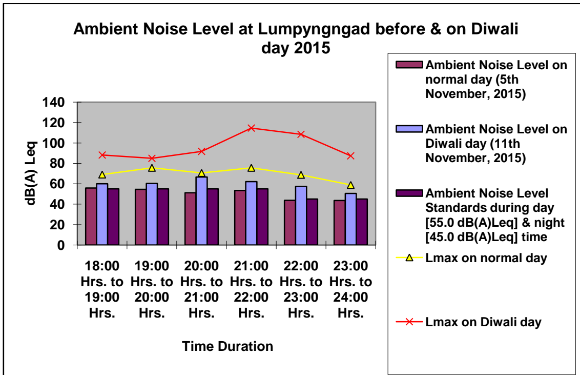
Fig. 1.0: Ambient Noise Level at Lumpynggad (Board’s Premises – Location A).
